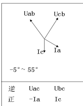
B、C相电压接反
